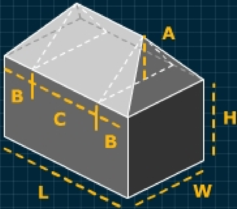
Pitched Roof, Two End Hips
